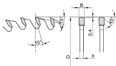
Main saw blade Lame de scie principale
